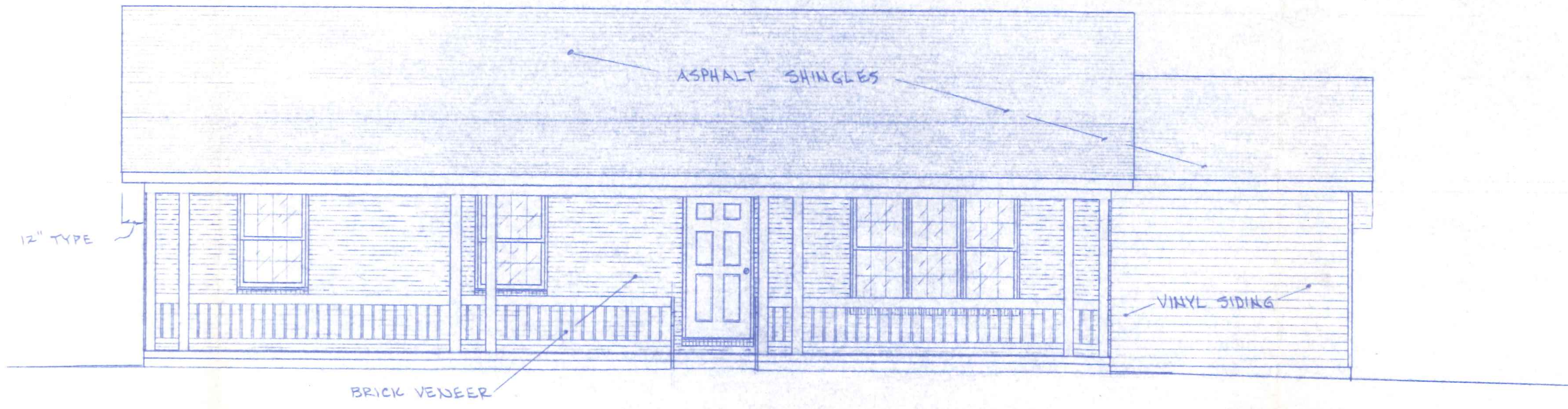
FRONT ELEVATION 1/4" = 1'-0"
